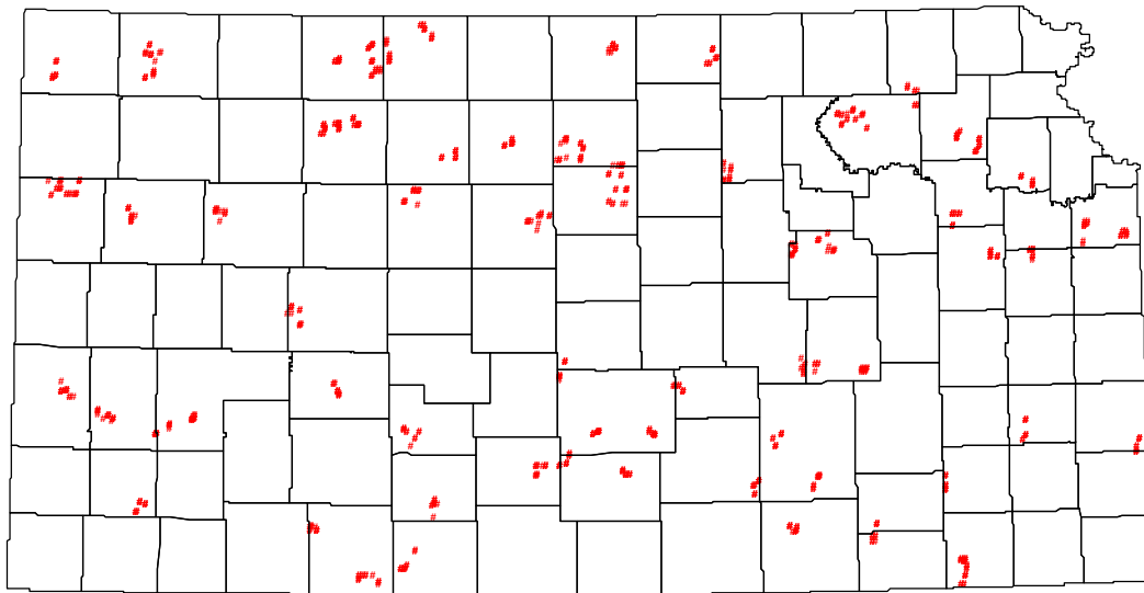
Figure 5. Field Verification Sites for Accuracy Assessment.
