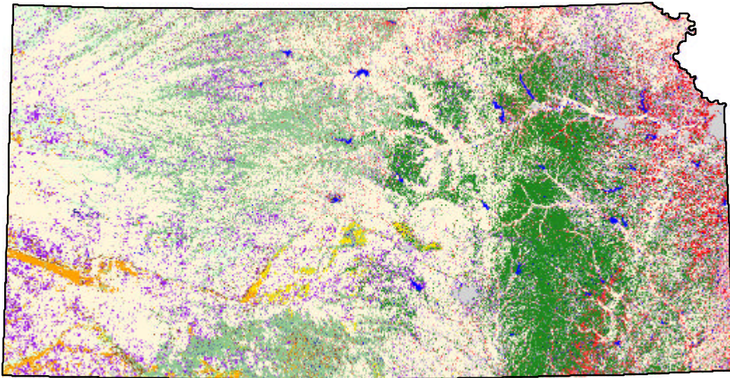
Figure 4. Final GAP Land Cover Map.
